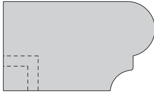
361 COUNTER EDGE 1.625 X 2.75 (.437 or .625 notch optional)
