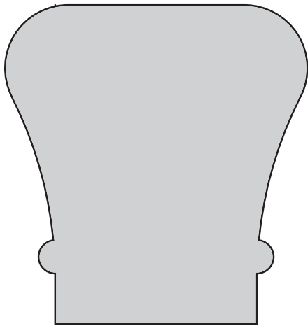
6312 HANDRAIL 2.375 X 2.250
