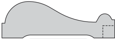
4500 CHAIR RAIL .75 X 2.375 (.25 X .25 notch is optional)
