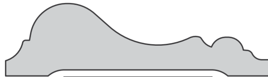
4520 CHAIR RAIL .75 X 2.750
