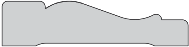
2050 CASING .75 X 3.125
