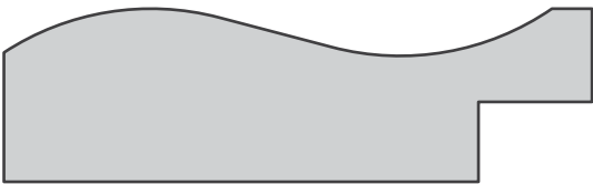
6075 FURNITURE BASE .812 X 2.750 w/ .375 X .531 NOTCH
