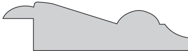
3216 BASE CAP .812 X 3.125
