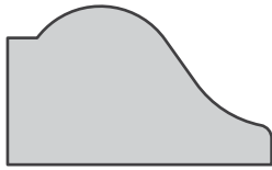
3213 BASE CAP .75 X 1.250
