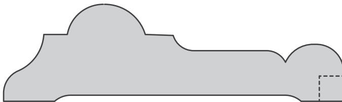
4528 CHAIR RAIL 1.00 X 3.500 (.25 X .25 notch is optional)
