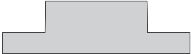
6069 GOBLET RAIL - NEW .937 X 3.312
