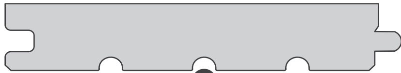
6307 FLOORING .750 X up to 8.25
