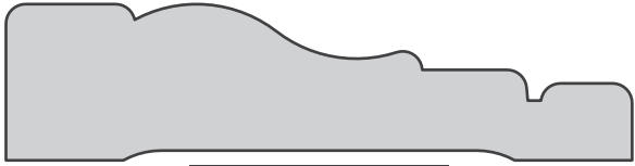
2046 CASING .75 X 3.00
