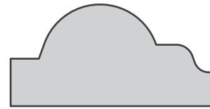
4531 CHAIR RAIL .75 X 1.5
